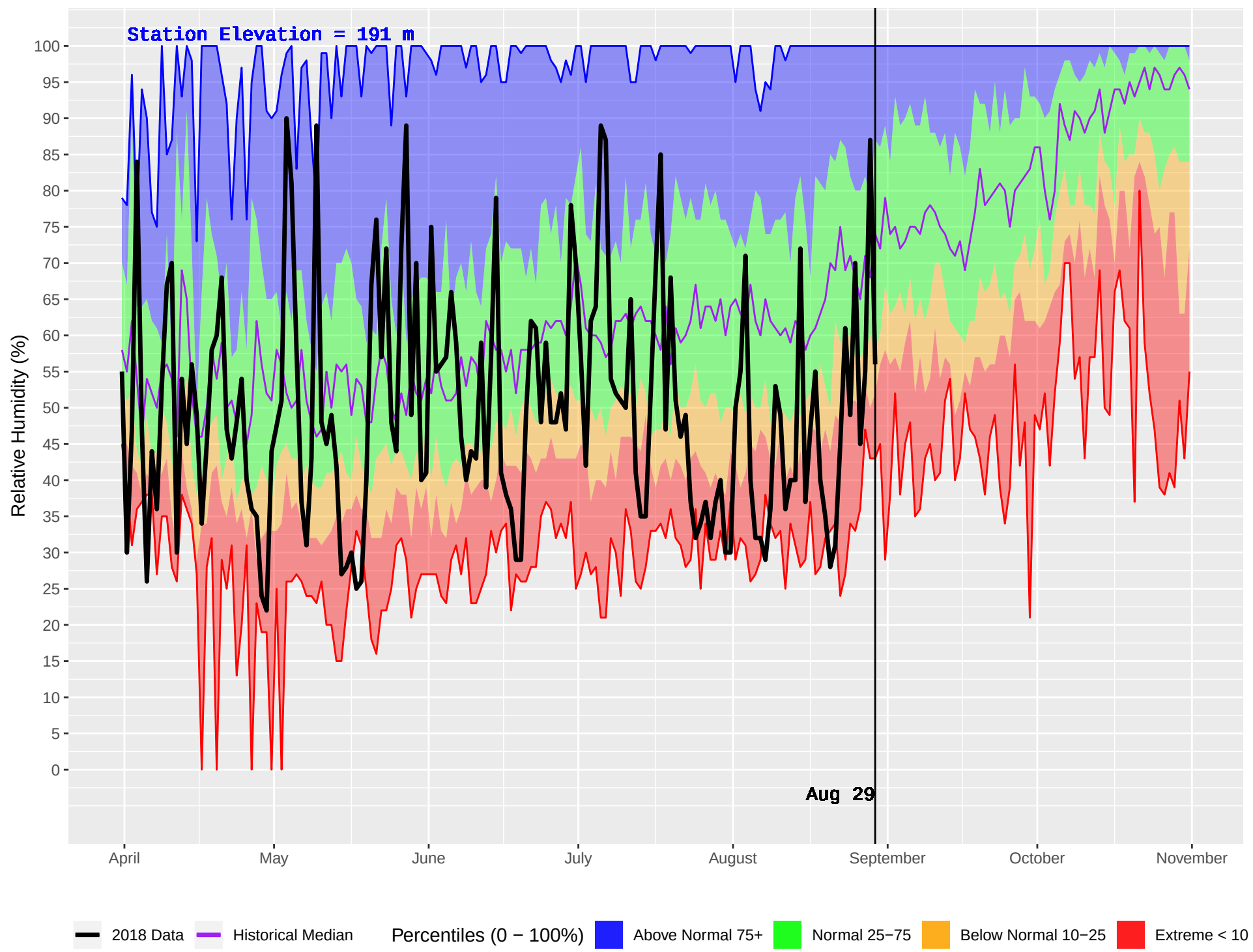
NASS CAMP (427) : Historical (1970–2016) and Current (2018) Daily Relative Humidity
